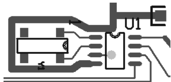
FIGURE 19. SUGGESTED LAYOUT FOR ISL12022 AND CRYSTAL
