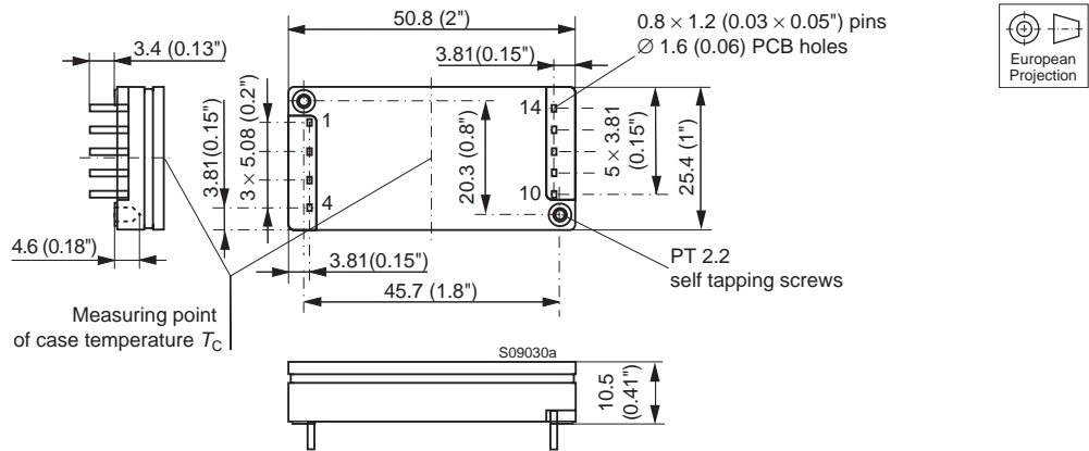
Fig. 18 Case IMX7/IMS7 with standard pinout
