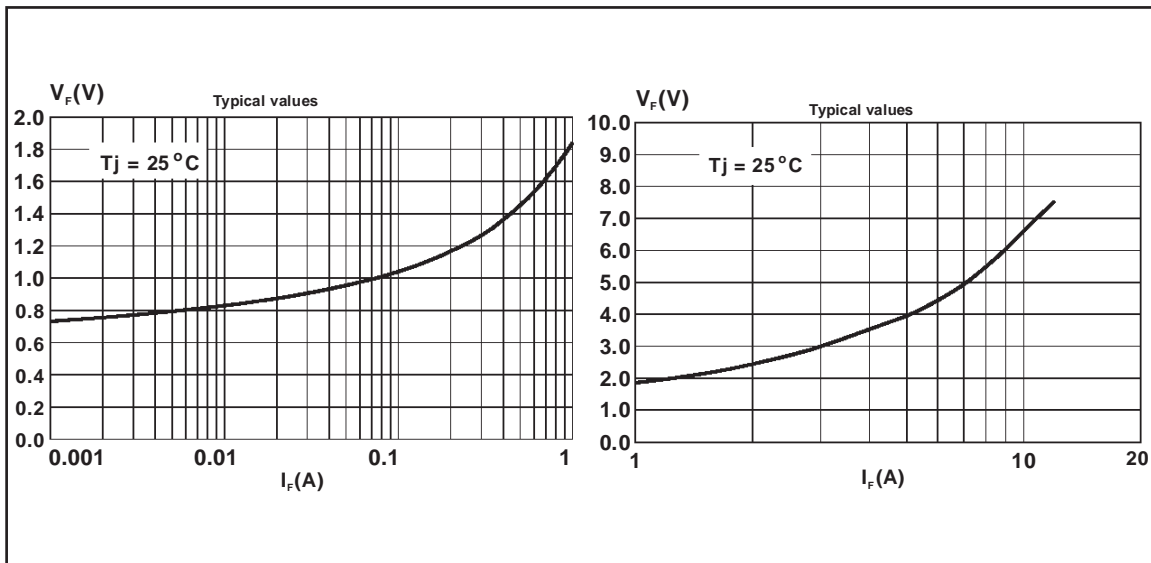
Fig.2 : Typical peak forward voltage characteristics (8/20 \mu\text{s} pulse)
