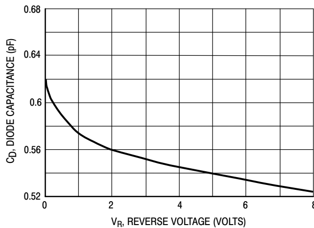
Figure 4. Diode Capacitance
