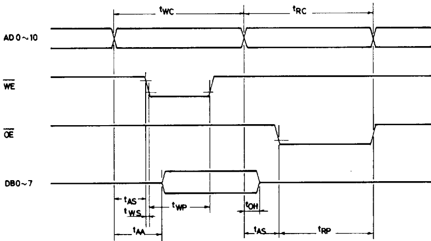
Fig.4 RAM Access
