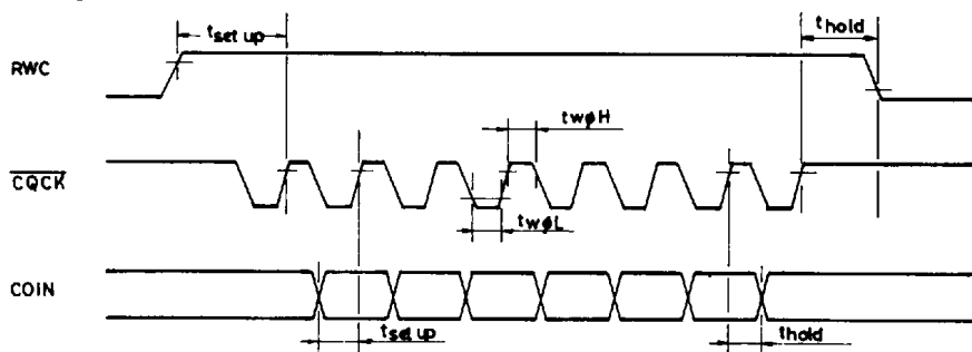
Fig.1 Command Input
