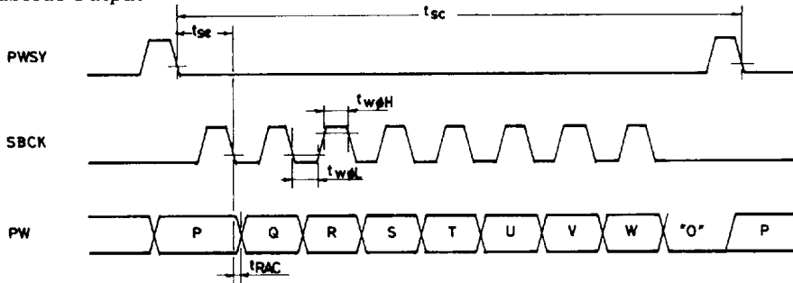
Fig.3 Subcode Output
