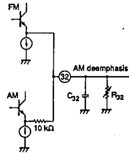
Figure 31. AM level
