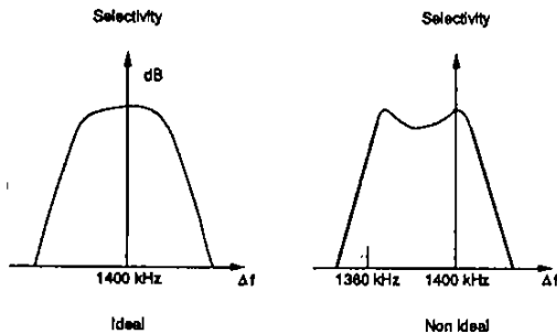
Figure 32. Tracking characteristic
