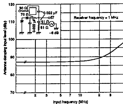
Figure 27. Detector AGC frequency response
