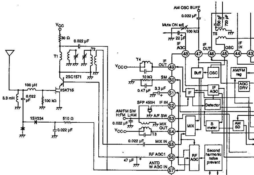
Figure 21. AGC stage
