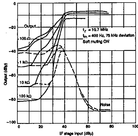
Figure 12. Muting attenuation characteristics
