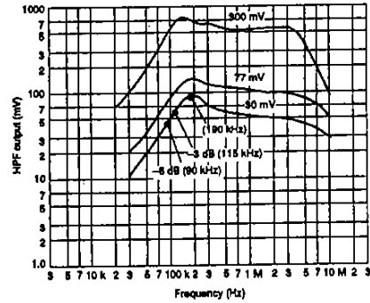
Pin 8 output vs. frequency (1)
