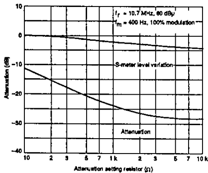
Figure 14. Muting attenuation's resistor dependence
