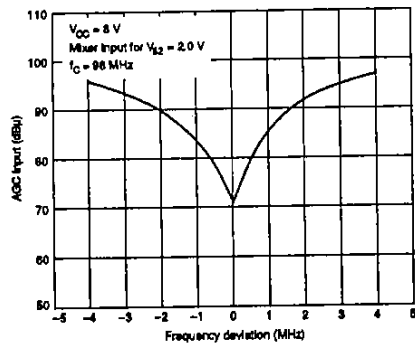
Figure 3. Input characteristic
