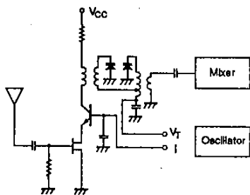
Figure 25. Second-harmonic beat noise generation
