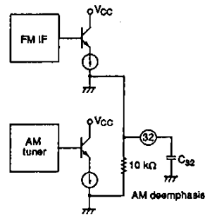
Figure 20. Equivalent output circuit
