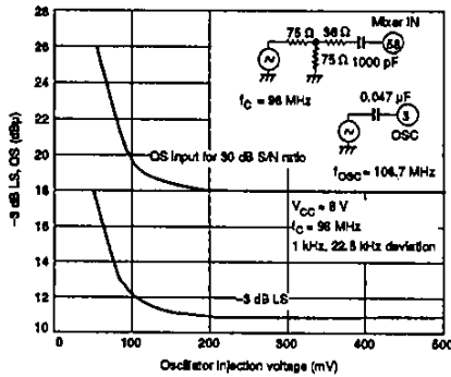
Figure 5. Mixer gain vs. oscillator output
