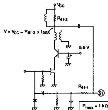
Figure 28. AGC ON level adjustment
