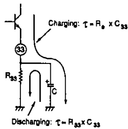
Figure 9. Mute drive time constant
