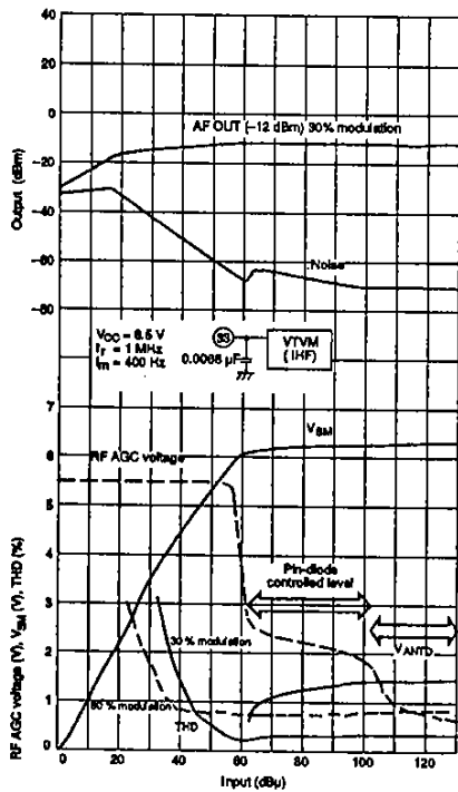
Figure 22. AM stage characteristics
