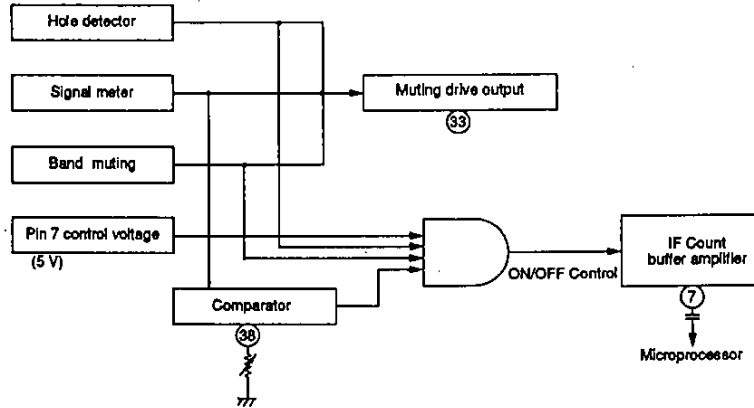
Figure 8. IF count buffer
