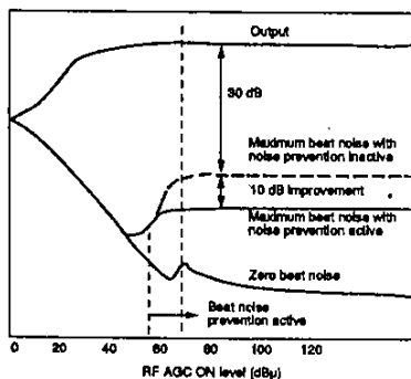
Figure 26. Beat noise suppression
