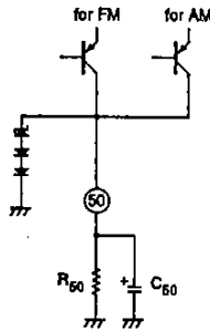
Figure 19. S-meter output
