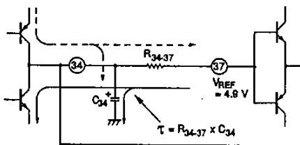
Figure 10. AFC input time constant
