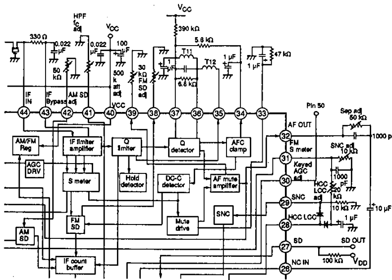
Figure 7. FM IF stage
