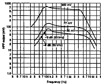
High-pass filter frequency response (mono)
