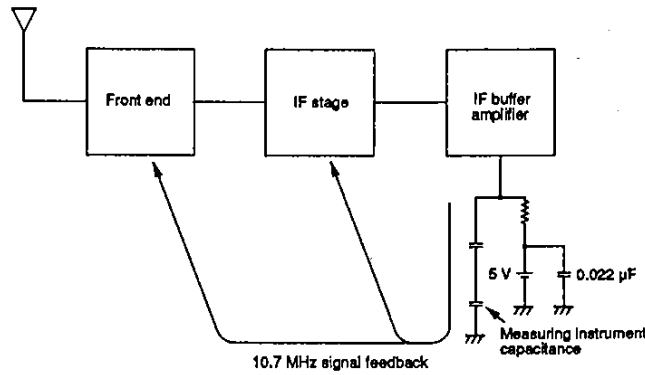
Figure 18. IF count feedback
