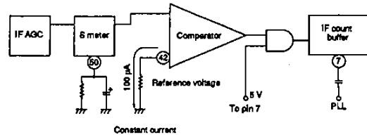
Figure 30. Station seek system
