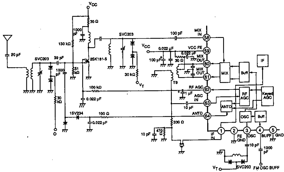
Figure 1. AGC stage
