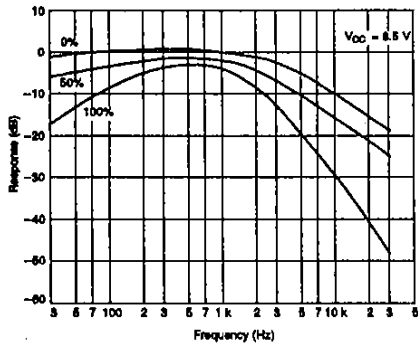
Low-pass filter frequency response (2)
