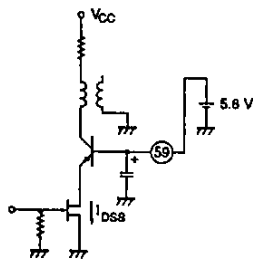
Figure 29. Cascade transistor
