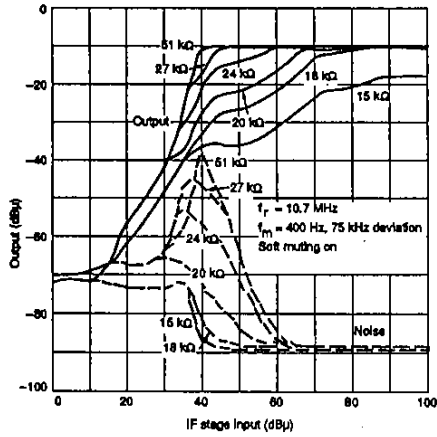
Figure 13. Muting ON level characteristics
