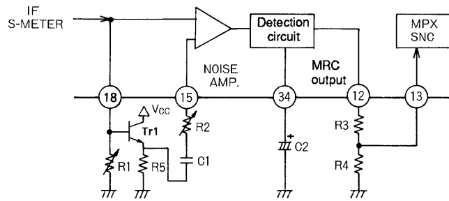
Figure 4 Application Circuit Using IF S-Meter High-Area Detection
