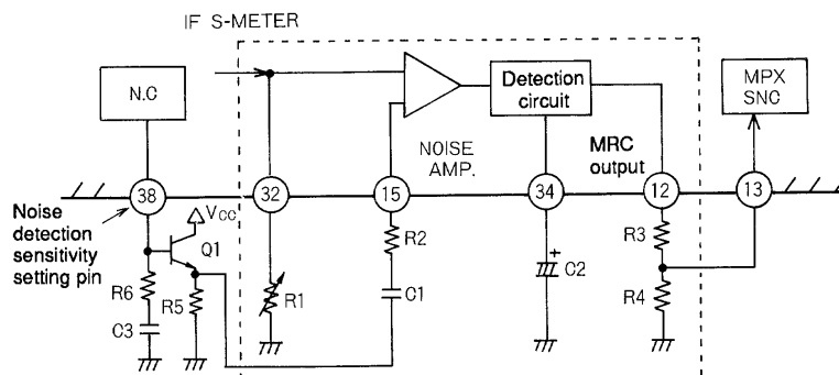
Figure 3 Application Circuit Using NC HPF Noise Detection
