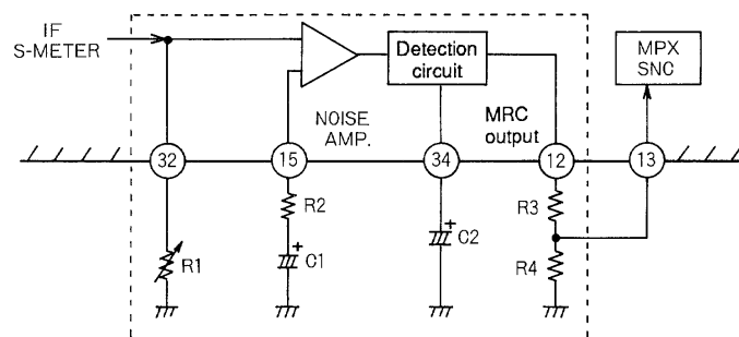
Figure 2 Multipath Circuit
