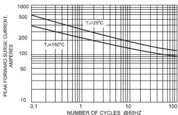
FIG.2 - NON - REPETITIVE PEAK FORWARD SURGE CURRENT
