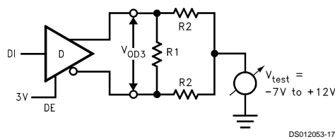
FIGURE 2. Driver V_{OD3}
