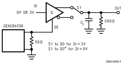
FIGURE 7. TRI-STATE and Sleep Mode Test Circuit ( t_{PZH} , t_{PSH} , t_{PHZ} )
