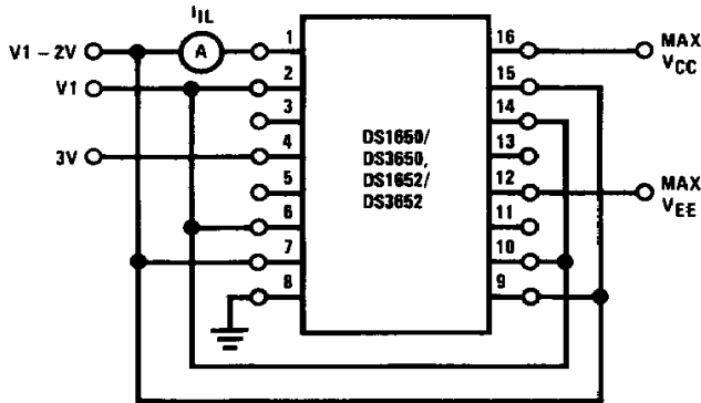
FIGURE 6. I_{IL}
