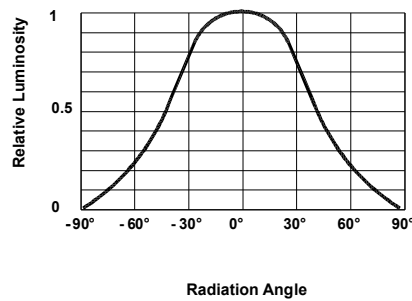
Fig 5. Radiation Diagram
