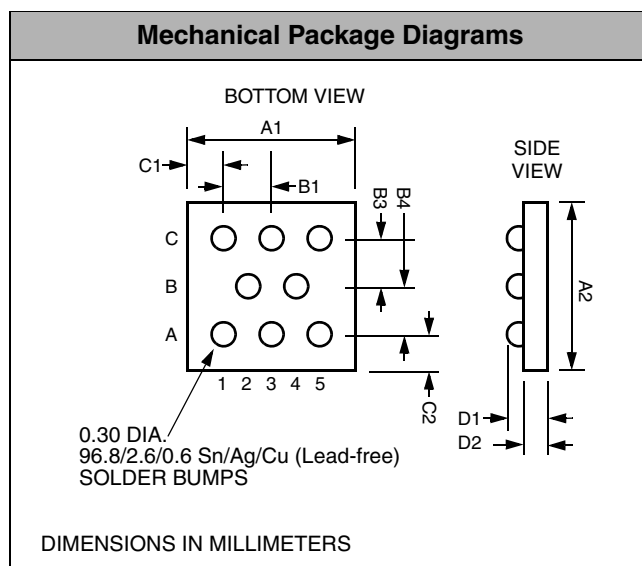
Package Dimensions for CSPEMI205 Chip Scale Package
