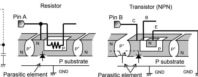
Fig.28 Simplified structure of monolithic IC
