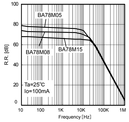
Fig.9 Ripple Rejection Ratio
