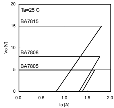
Fig.17 Load Regulation
