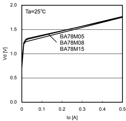
Fig.7 Dropout Voltage
