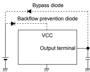
Fig.27 Bypass Diode
