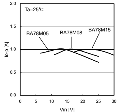
Fig.6 Peak Output Current
