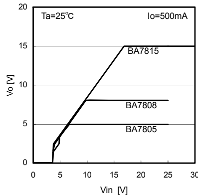
Fig.14 Line Regulation (Io=500mA)
