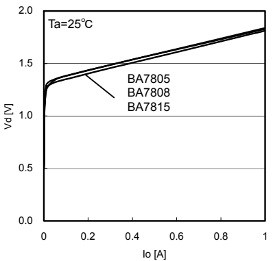
Fig.19 Dropout Voltage
