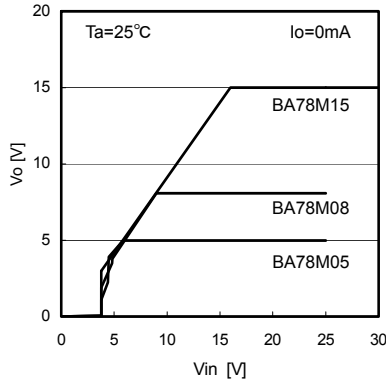
Fig.1 Line Regulation (Io=0mA)
