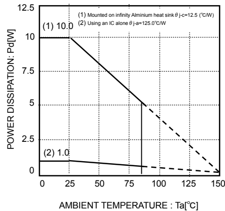
Fig.26 Thermal derating curve (TO252-3)
