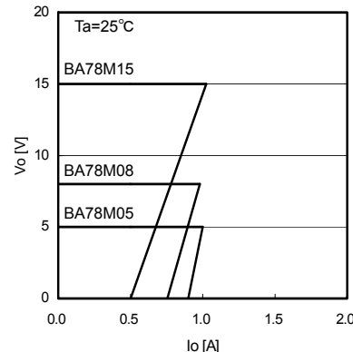
Fig.5 Load Regulation
