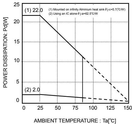
Fig.25 Thermal derating curve (TO220CP-3)
