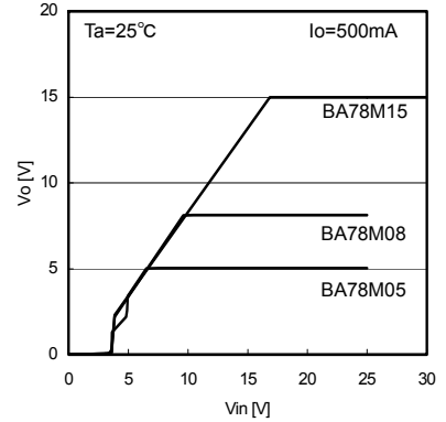
Fig.3 Line Regulation (Io=500mA)
