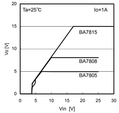
Fig.15 Line Regulation (Io=1A)
