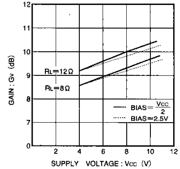
Fig. 10 Driver supply voltage vs. voltage gain
