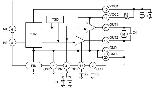
Fig.13 BA6219BFP-Y
