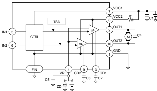
Fig.15 BA6222
