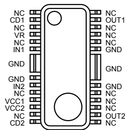
Fig.14 HSOP25
