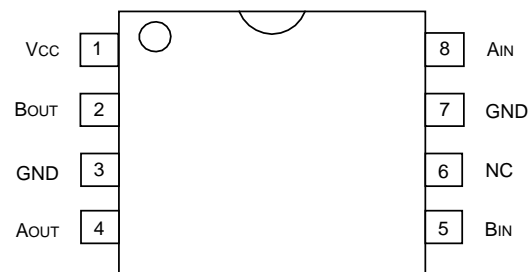
For SOP-8/DIP-8 Package
