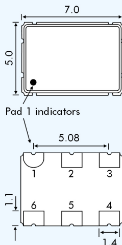
Pad Connections HP_5761
