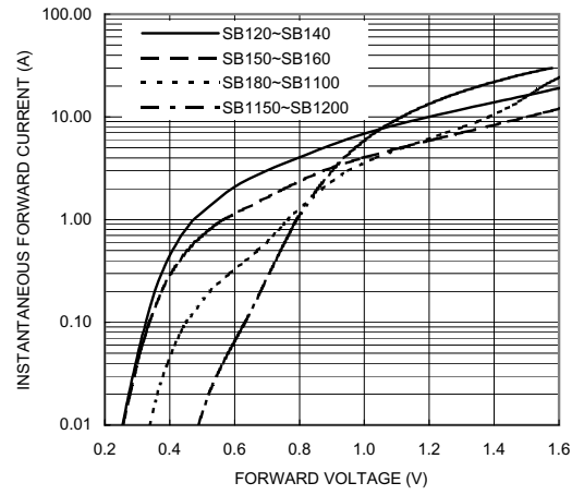
FIG. 2-TYPICAL FORWARD CHARACTERISTICS
