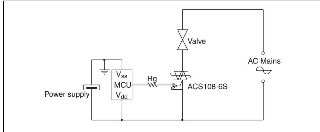
Figure 13. Typical application program
