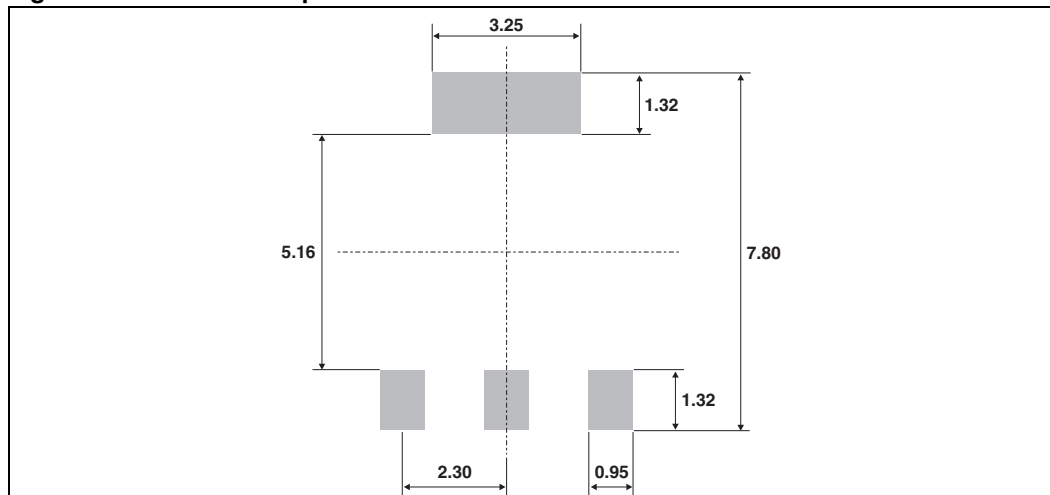
Figure 18. SOT-223 Footprint
