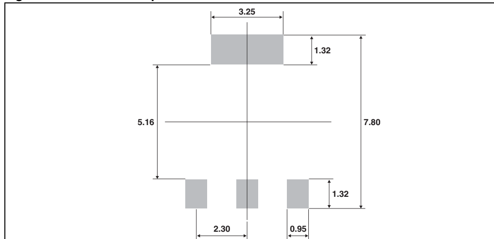
Figure 18. SOT-223 Footprint
