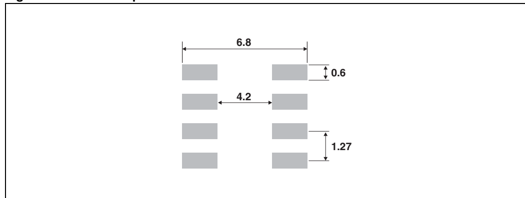
Figure 18. SO-8 Footprint
