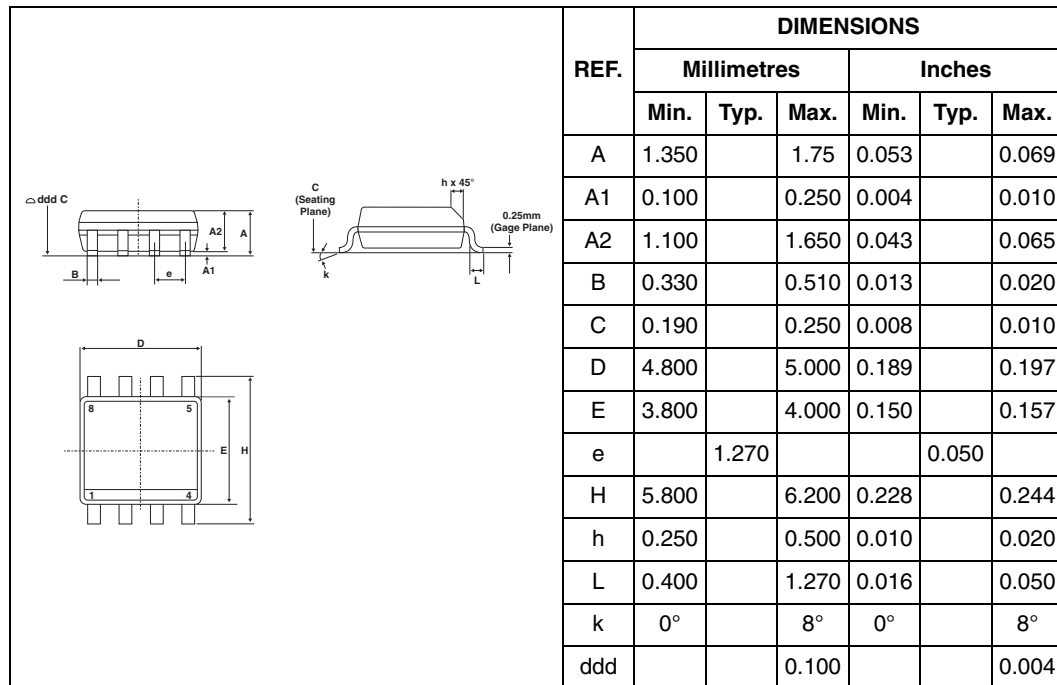
Figure 18. SO-8 Footprint
