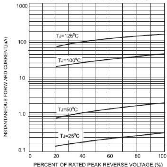
FIG.5-TYPICAL REVERSE CHARACTERISTICS
