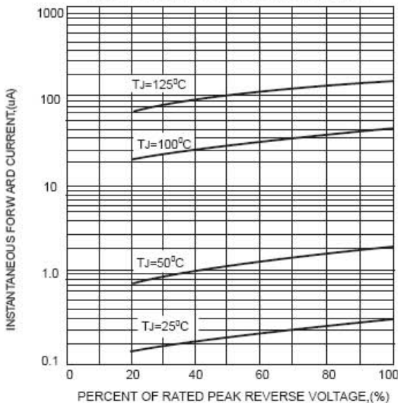
FIG.5-TYPICAL REVERSE CHARACTERISTICS
