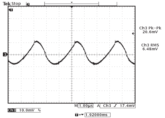
Figure 16: Typical Ripple and Noise* (Channel 3: Vo)
