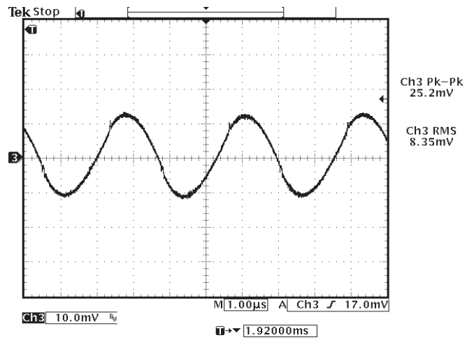
Figure 8: Typical Ripple and Noise* (Channel 3: Vo)
