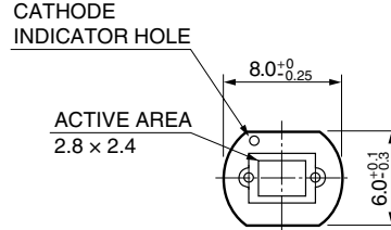
④ S1133-01/-14
