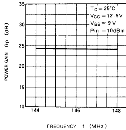
POWER GAIN VS. FREQUENCY
