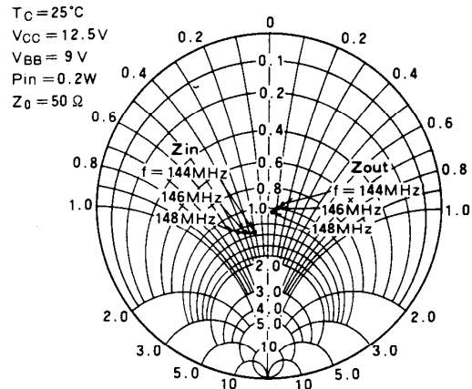
INPUT IMPEDANCE, OUTPUT IMPEDANCE VS. FREQUENCY
