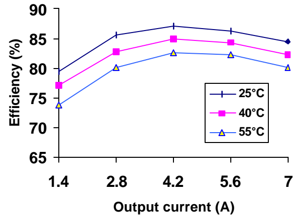
Fig 12. Efficiency at nominal input (48V) vs. load at different ambient temperatures of 25^{\circ}C , 40^{\circ}C , 55^{\circ}C without air flow, the input voltage is 48V.
