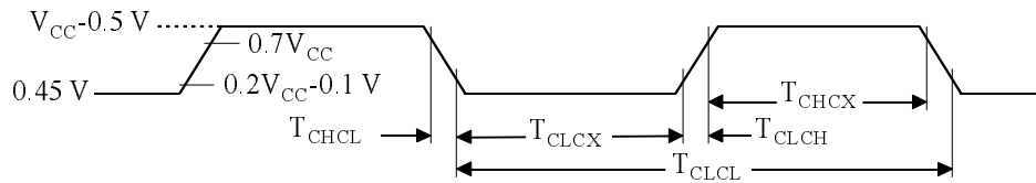
Figure 19-11. External Clock Drive Waveforms
