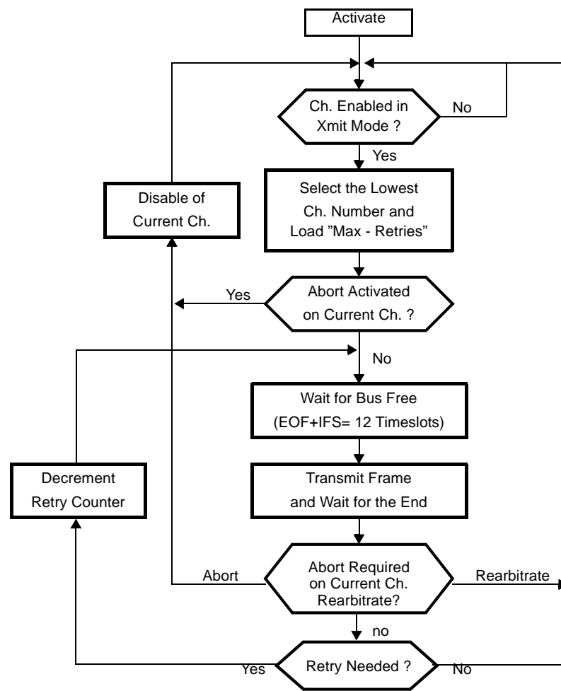
Figure 30. Transmit Function
