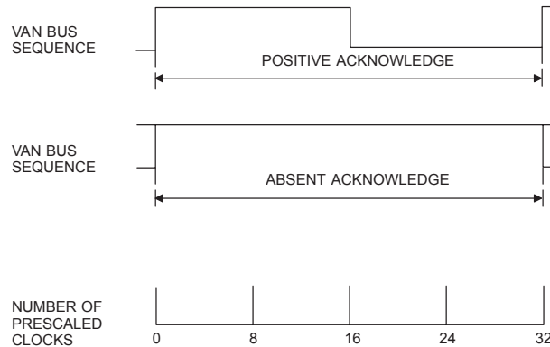
Figure 16. Acknowledge Sequences
