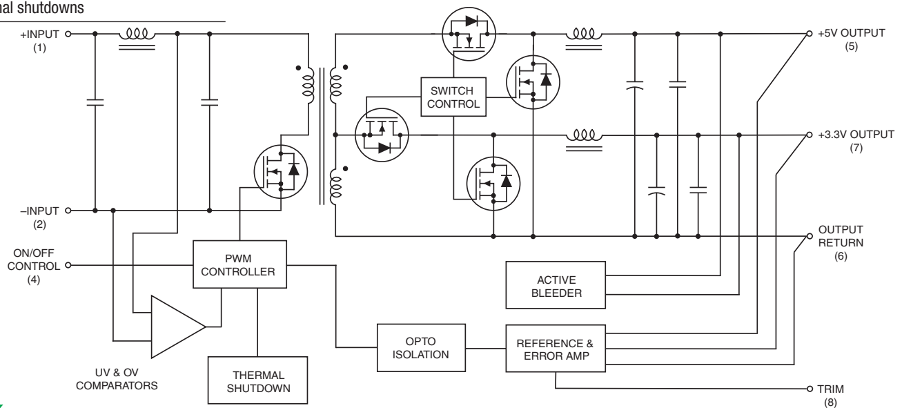
Figure 1. Simplified Schematic
