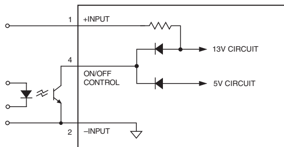
Figure 2. Driving the Positive Polarity On/Off Control Pin
