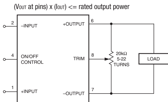
Figure 5. Trim Connections Using A Trimpot
