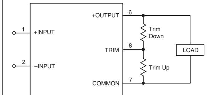
Figure 2b. Trim Connections Using Fixed Resistors
