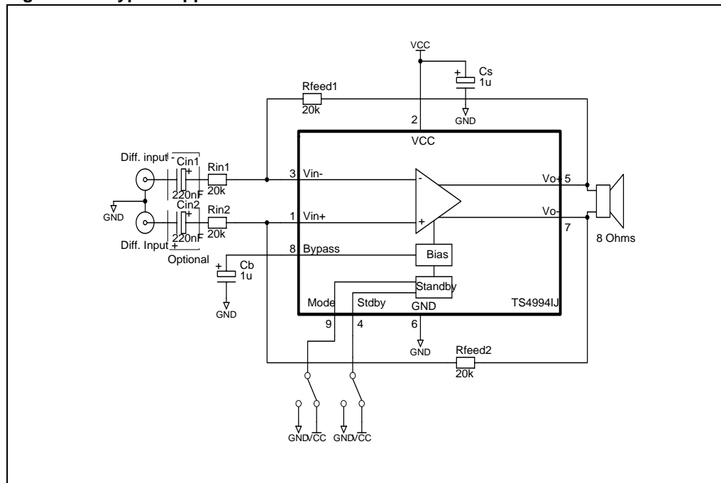
Figure 1. Typical application
