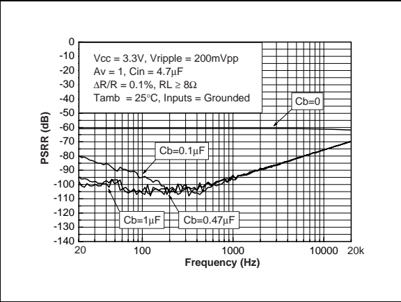
Figure 90. PSRR vs. frequency (worst case conditions)
