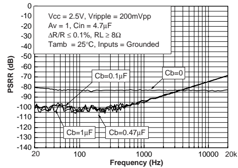
Figure 93. PSRR vs. frequency with random choice condition
