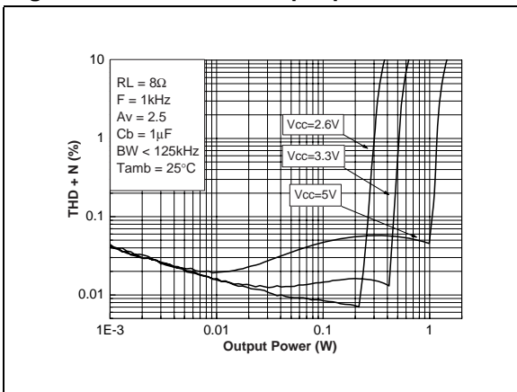
Figure 54. THD+N vs. output power
