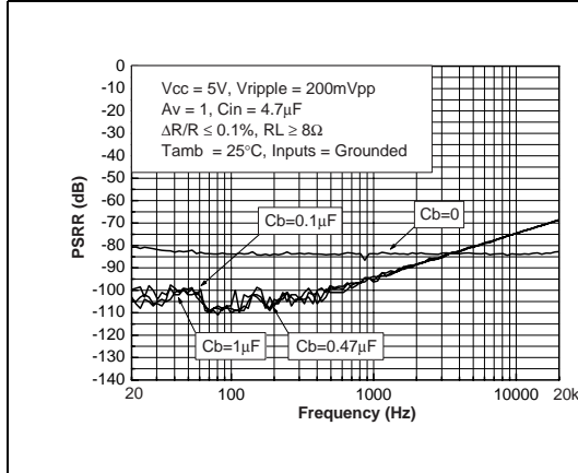
Figure 92. PSRR vs. frequency with random choice condition
