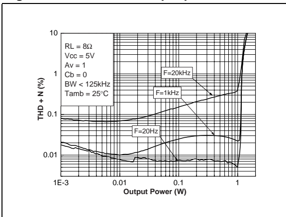
Figure 78. THD+N vs. output power
