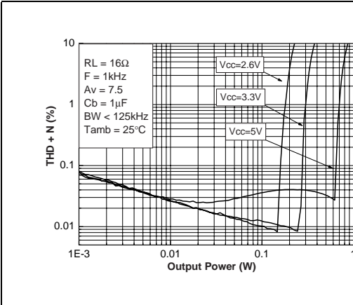
Figure 58. THD+N vs. output power
