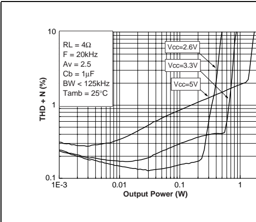
Figure 60. THD+N vs. output power
