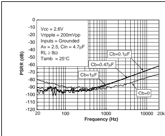
Figure 28. PSRR vs. frequency
