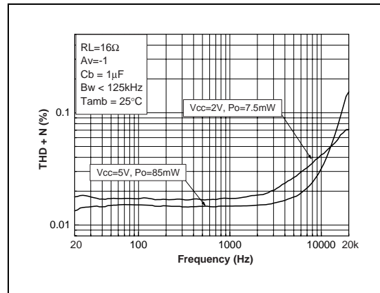
Fig. 42: THD + N vs Frequency
