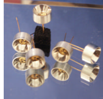
Package TO-18 with reflector
