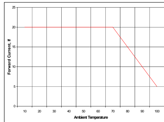
Maximum forward current vs. temperature.
