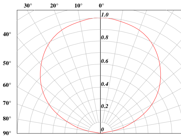
Radiation pattern.
