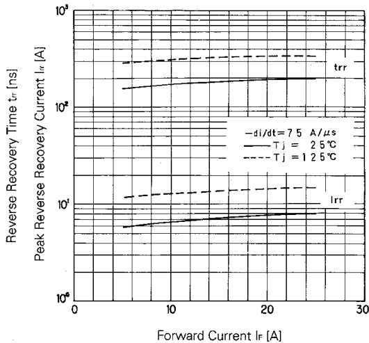
T_{rr}, I_{rr} - I_f
