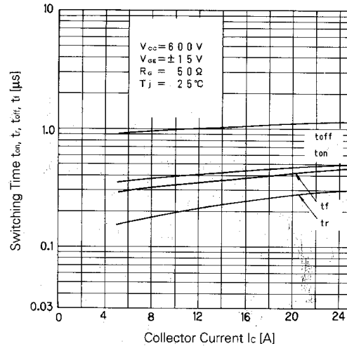
Switching Time
