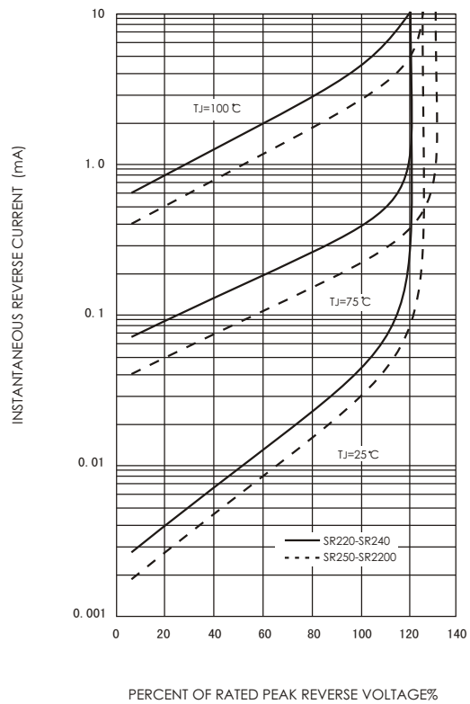
FIG.4-TYPICAL REVERSE CHARACTERISTICS
