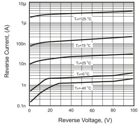
Fig.2 - Reverse Characteristics
