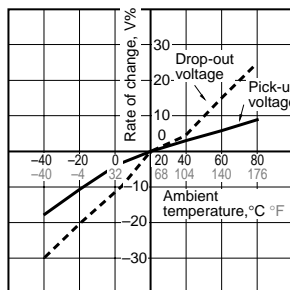
Tested sample: DE2a-5V, Ambient temperature: -40°C to 80°C -40°F to 176°F, Quantity: n=6
