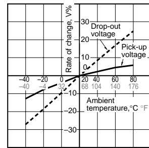
Tested sample: DE1a-5V, Ambient temperature: -40°C to 80°C -40°F to 176°F, Quantity: n=6
