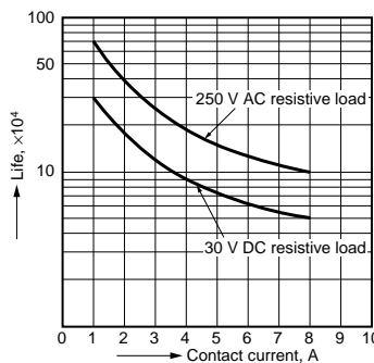
2.-(3) Life curve (2 Form A)
