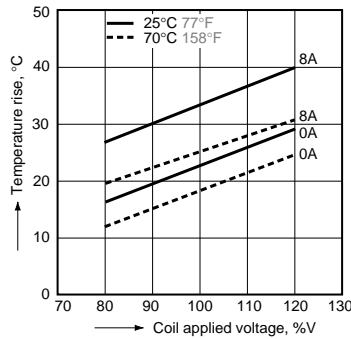
3.-(3) Coil temperature rise (2 Form A) Tested sample: DE2a-5V Quantity: n=6 Ambient temperature: 25°C to 70°C 77°F to 158°F
