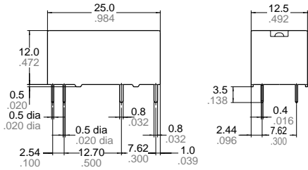
2 coil latching type
