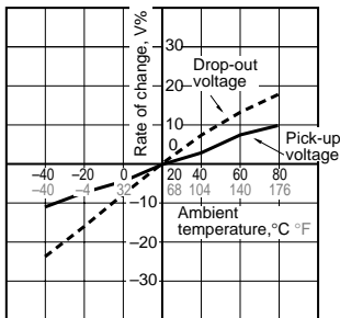
Tested sample: DE1a1b-5V, Ambient temperature: -40°C to 80°C -40°F to 176°F, Quantity: n=6
