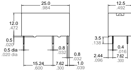
Single side stable 1 coil latching type
