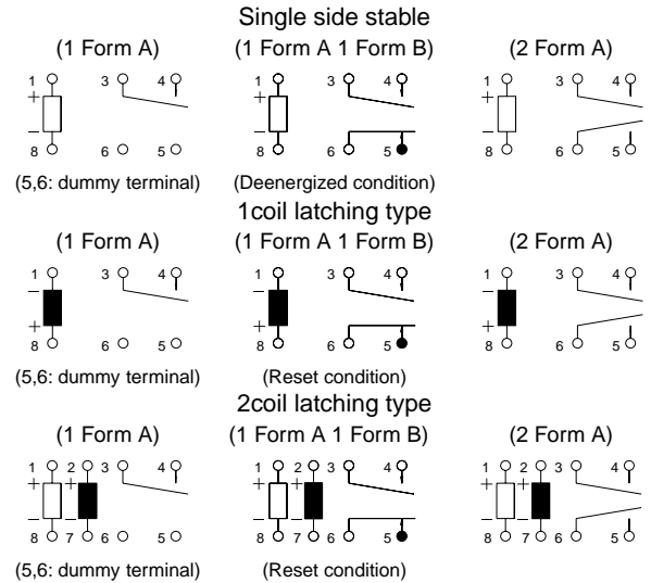
Schematic (Bottom view)
