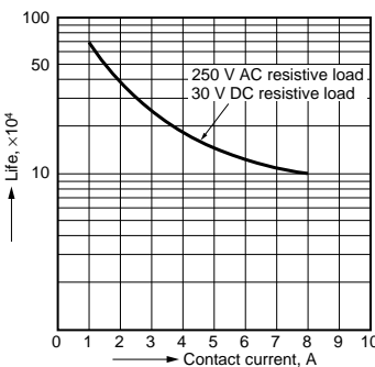
2.-(2) Life curve (1 Form A 1 Form B)
