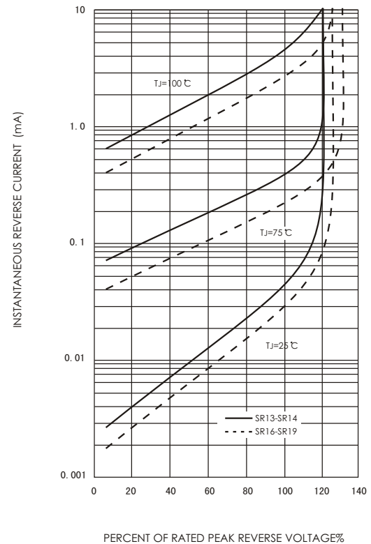
FIG.4-TYPICAL REVERSE CHARACTERISTICS
