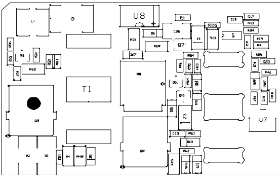
the hottest component Q5 on top view
