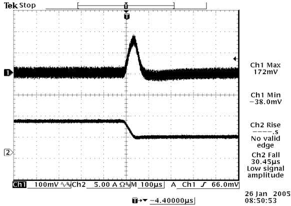
50%-75% Load Transients at Vin=48 V
