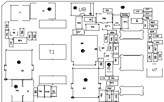
Temperature reference points on top side
