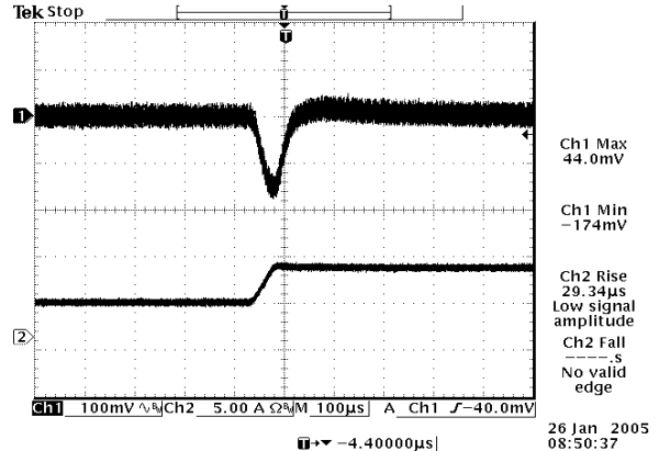
75%-50% Load Transients at Vin=48 V
