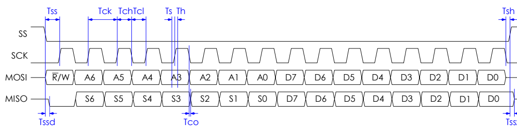
Figure 3 Serial peripheral interface timing
