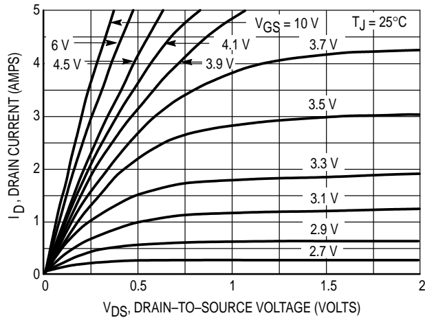
Figure 3. On-Region Characteristics
