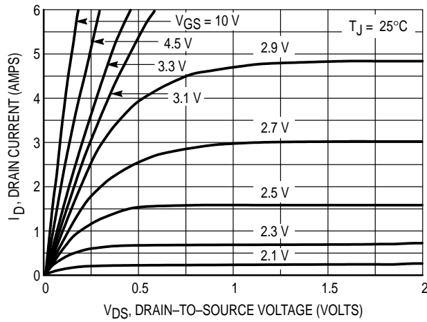
Figure 3. On-Region Characteristics
