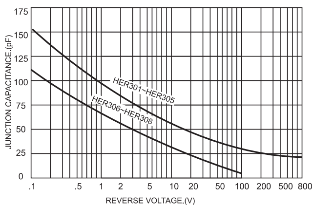
FIG.6-TYPICAL JUNCTION CHARACTERISTICS
