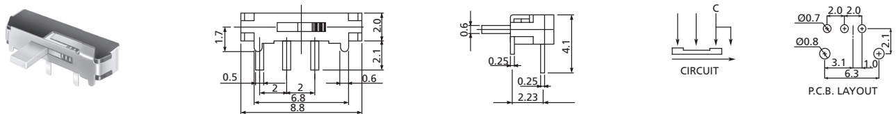
SB3HR THT Terminals, with Spring Return
