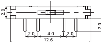
SB4H1 Thru Hole Type Terminals
