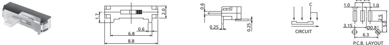
SB3SR SMT Terminals, with Spring Return
