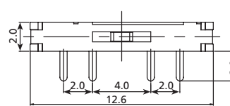
SB4H2 Thru Hole Type Terminals
