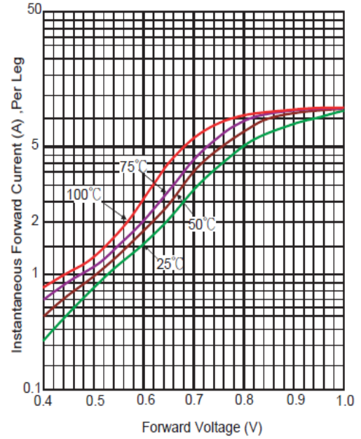
Typical Forward Characteristic
