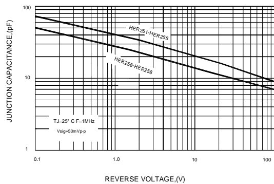
FIG.5-TYPICAL JUNCTION CAPACITANCE
