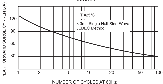
FIG.5-MAXIMUM NON-REPETITIVE SURGE CURRENT
